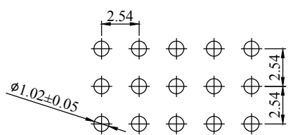
Recommended P.C.Board Hold Layout
