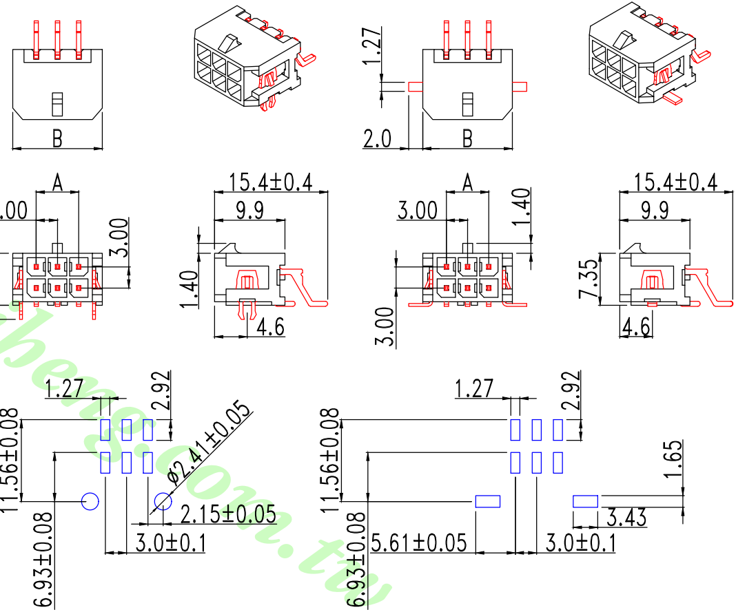
PCB Layout: Component side
