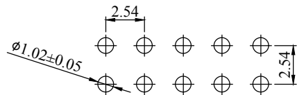
Recommended P.C.Board Hold Layout
