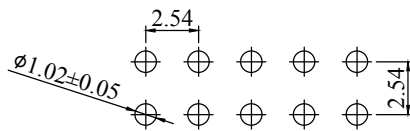
Recommended P.C.Board Hold Layout
