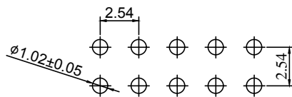
Recommended P.C.Board Hold Layout
