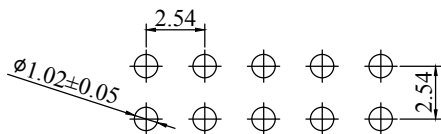
Recommended P.C.Board Hold Layout
