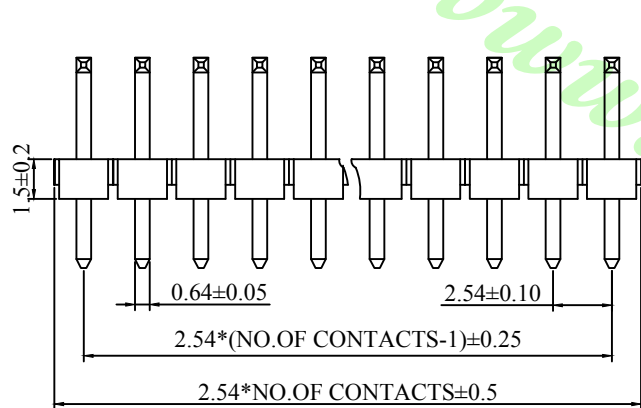
Pin Chart:
