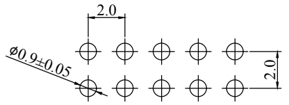
Recommended P.C.Board Hold Layout
