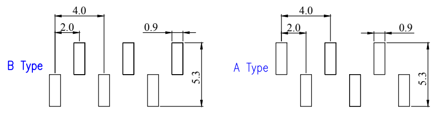
Recommended P.C.Board Hold Layout
