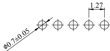
Recommended P.C.Board Hold Layout
