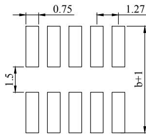
Recommended P.C.Board Hold Layout
