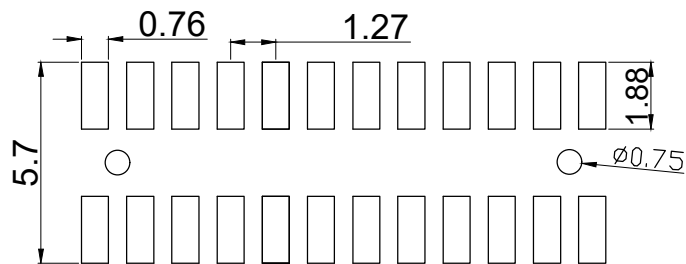
P. C. B Layout
