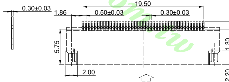
FPC/FFC Insert Direction Recommended P.C.B Layout
