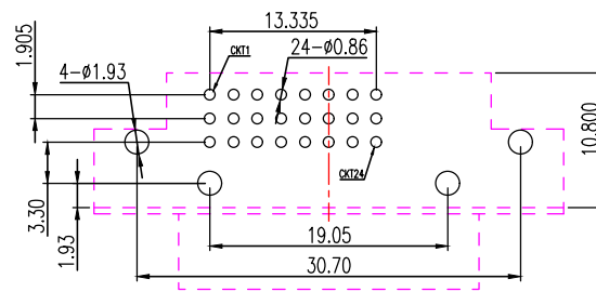
RECOMMENDED P.C.B LAYOUT INSPECTION DIMENSION:(A)~(H)
