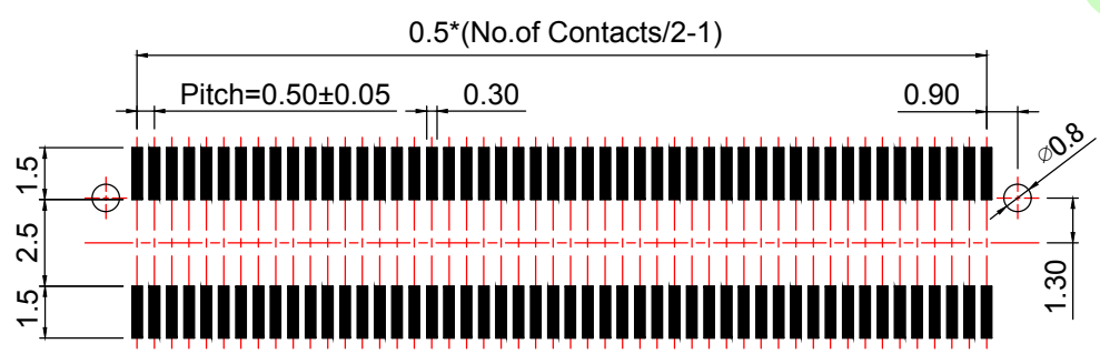
PCB Layout For Surface Mounting
