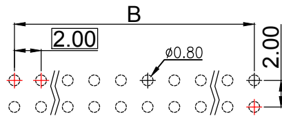
PCB Layout (Top View)
