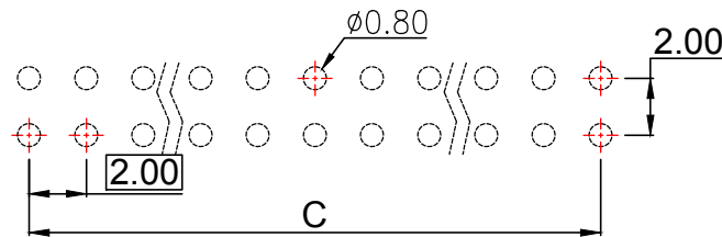
PCB Layout (Top View)
